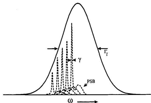
Figure 2. Schematic representation of homogeneous ( \gamma ) and inhomogeneous ( \Gamma_I ) broadening. Profiles of the zero-phonon lines (ZPL) and their associated sidebands (PSB) for specific frequencies have been enlarged compared to the inhomogeneous line to provide more detail. Reprinted from ref 7. Copyright 1992 Kluwer Academic Publishers.
