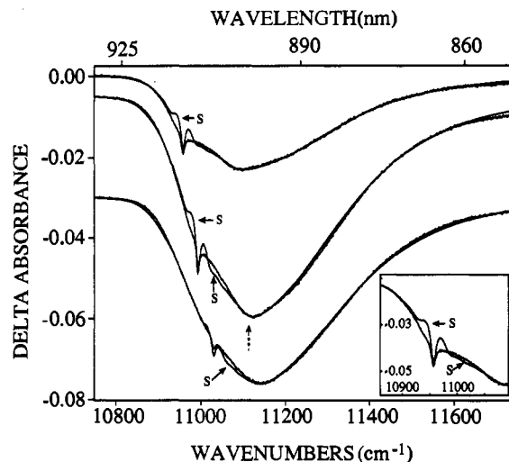
Figure 17. PHB spectra of P870 (protonated, R-26) for \omega_B = 10\,921 , 10\,992 , and 11\,039\text{ cm}^{-1} (top to bottom), T = 4.2\text{ K} . Simulations (S) of these spectra were obtained with the parameter values of Table VIII. The dashed arrow indicates the position where the satellite ZPH of \omega_{ap}^1 would occur if the marker mode were not damped, cf. text. The inset is a blowup of the region around the ZPH for the upper spectrum. Reprinted from ref 238. Copyright 1993 American Chemical Society.
