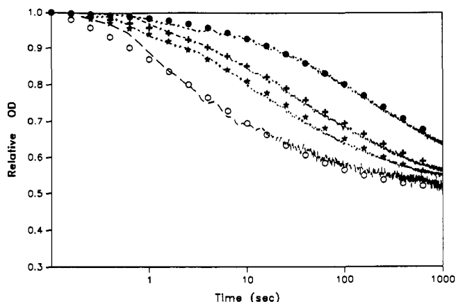
Figure 15. Hole growth curves of cresyl violet in PVOH at 1.6 K for different burn intensities, I_B = 3, 15, 30, and 200 \mu\text{W}/\text{cm}^2 (from top to bottom). The dots, crosses, stars, and circles represent theoretical fits. For all simulations, a single set of parameters, \lambda_0 = 9.85 , \sigma_2 = 1.3 , \Omega_0 = 10^{12} \text{ s}^{-1} , \sigma = 2 \times 10^{-11} \text{ cm}^2 , and S = 0.7 , were used. The OD of sample is \sim 0.35 (at 632.8 \text{ nm} , He-Ne line). Reprinted from ref 151. Copyright 1992 Optical Society of America.
