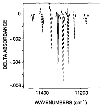
Figure 21. Constant fluence ( 250 \text{ mW/cm}^2 for 30 min) hole-burned spectra in "B870" band. ZPHs are offset to have a common baseline and nonresonant holes accompanying the ZPHs are not shown. The maximum absorbance change shown is \sim 0.005 . Reprinted from ref 218. Copyright 1992 American Society of Photobiology.
