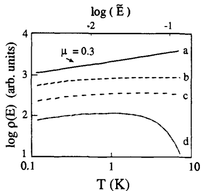
Figure 10. The density of states, \rho(E) , of the two-level systems (TLS int ) calculated with \lambda_0 = 7 , \Delta_0 = 0 , \sigma_\lambda = 2.5 , and different \bar{\sigma}_\Delta values; \bar{\sigma}_\Delta = 0.4 (curve b), \bar{\sigma}_\Delta = 0.2 (curve c), and \bar{\sigma}_\Delta = 0.05 (curve d). Curve a is a line with slope 0.3. \sigma_\Delta = \bar{\sigma}_\Delta(\hbar\omega_0) and \hbar\omega_0 = 4.96 \times 10^{-3} eV (40 cm -1 ).
