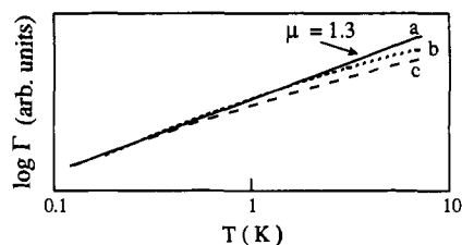
Figure 12. Temperature dependence of pure dephasing. Curve a is a line with slope \mu = 1.3 . Curves b and c were calculated for \Delta_0 = 0 , \lambda_0 = 7 , \sigma_\lambda = 2.5 , \bar{\sigma}_\Delta = 0.2 , and \hbar\omega_0 = 4.96 \times 10^{-3} eV. Curve b is the plot of \langle \Delta \rangle_E while curve c is the plot of \bar{E}\rho(\bar{E}) which yields T^{1+\mu} only for T < \sim 0.7 K.
