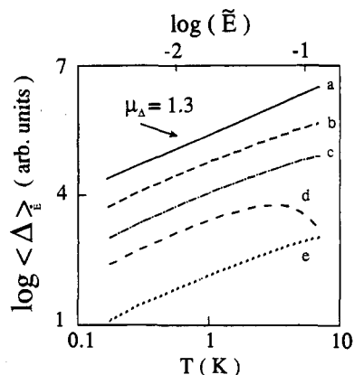
Figure 11. Average value of \langle \Delta \rangle_E as a function of reduced energy \bar{E} = E/\hbar\omega_0 (and T ) for \hbar\omega_0 = 4.96 \times 10^{-3} eV (40 cm -1 ) obtained for \lambda_0 = 7 , \Delta_0 = 0 , \sigma_\lambda = 2.5 and different values of \bar{\sigma}_\Delta : \bar{\sigma}_\Delta = 0.4 (curve b); \bar{\sigma}_\Delta = 0.2 (curve c); \bar{\sigma}_\Delta = 0.05 (curve d), respectively. Curve e was obtained for (\lambda_0, \Delta_0, \sigma_\lambda, \bar{\sigma}_\Delta) = (7, 0, 3, 0.2) . Curve a is a line with slope \mu_\Delta = 1.3 .
